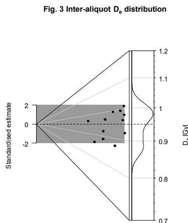
Fig. 3 Inter-aliquot D_e distribution
