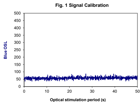
Fig. 1 Signal Calibration Natural blue and laboratory-induced infrared (IR) OSL signals. Detectable IR signal decays are diagnostic of feldspar contamination. Inset, the natural blue OSL signal (open triangle) of each aliquot is calibrated against known laboratory doses to yield equivalent dose ( D_e ) values. Repeats of low and high doses (open diamonds) illustrate the success of sensitivity correction.
