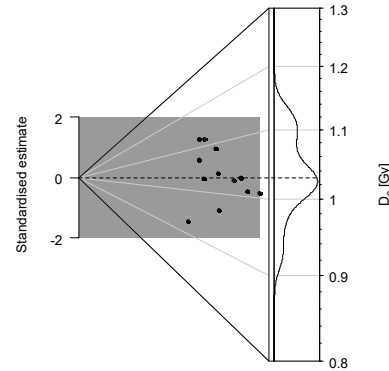
Fig. 3 Inter-aliquot D_e distribution
